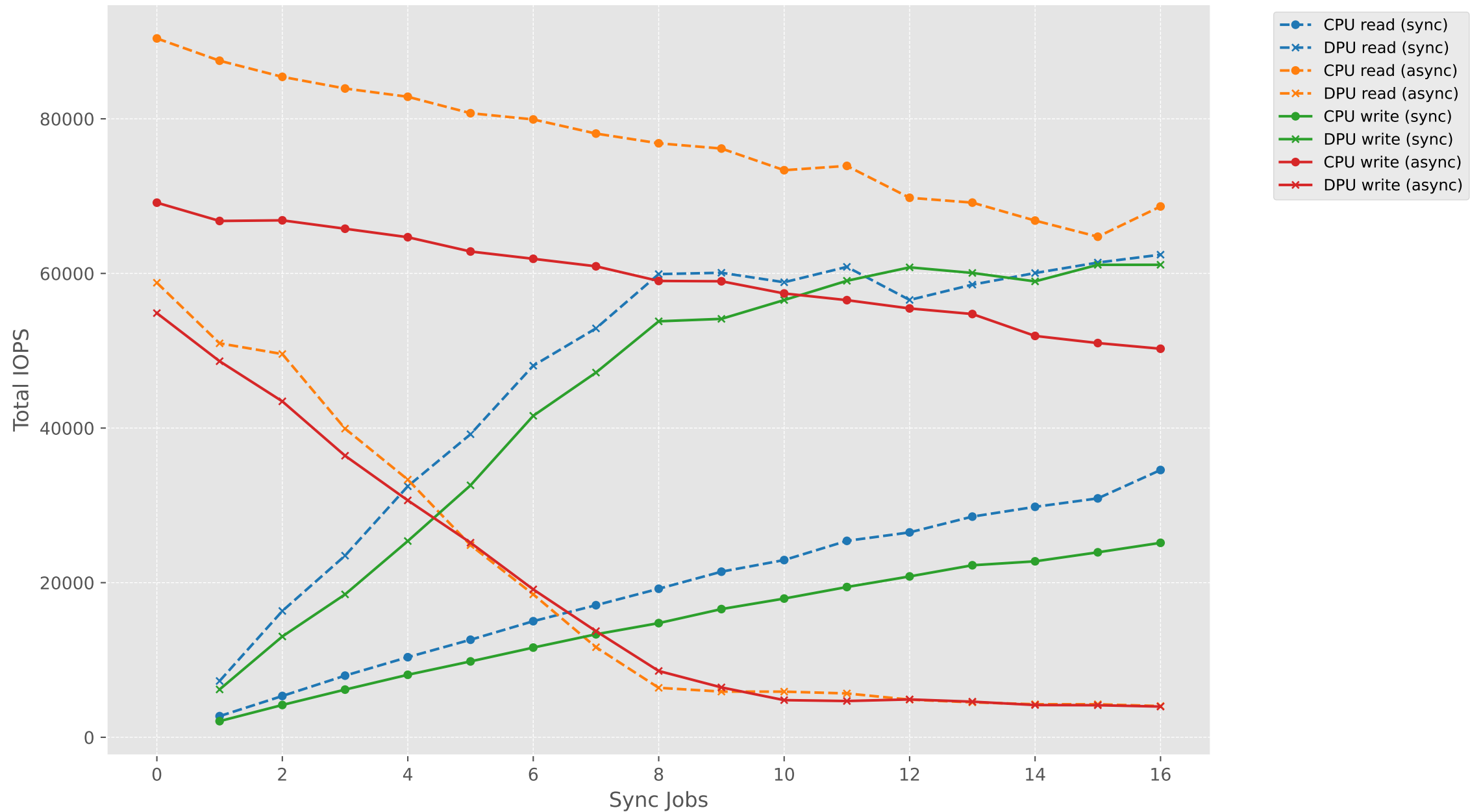
IOPS vs Sync Jobs (async1_syncN) - SEQ (CPU vs DPU)
